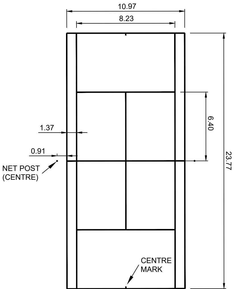
TYPICAL TENNIS COURT LINE MARKING SCALE 1 : 200
