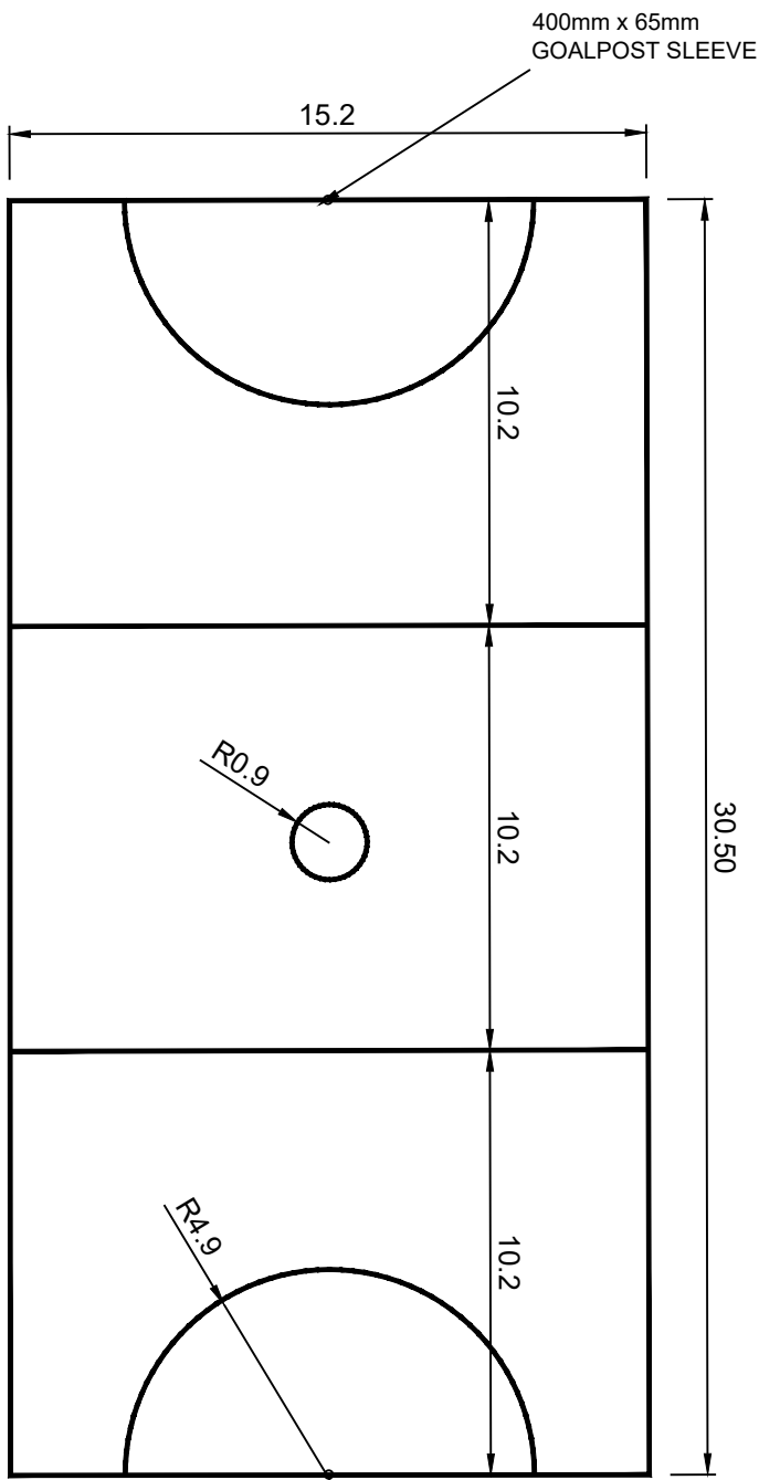
TYPICAL NETBALL COURT LINE MARKING SCALE 1 : 200
